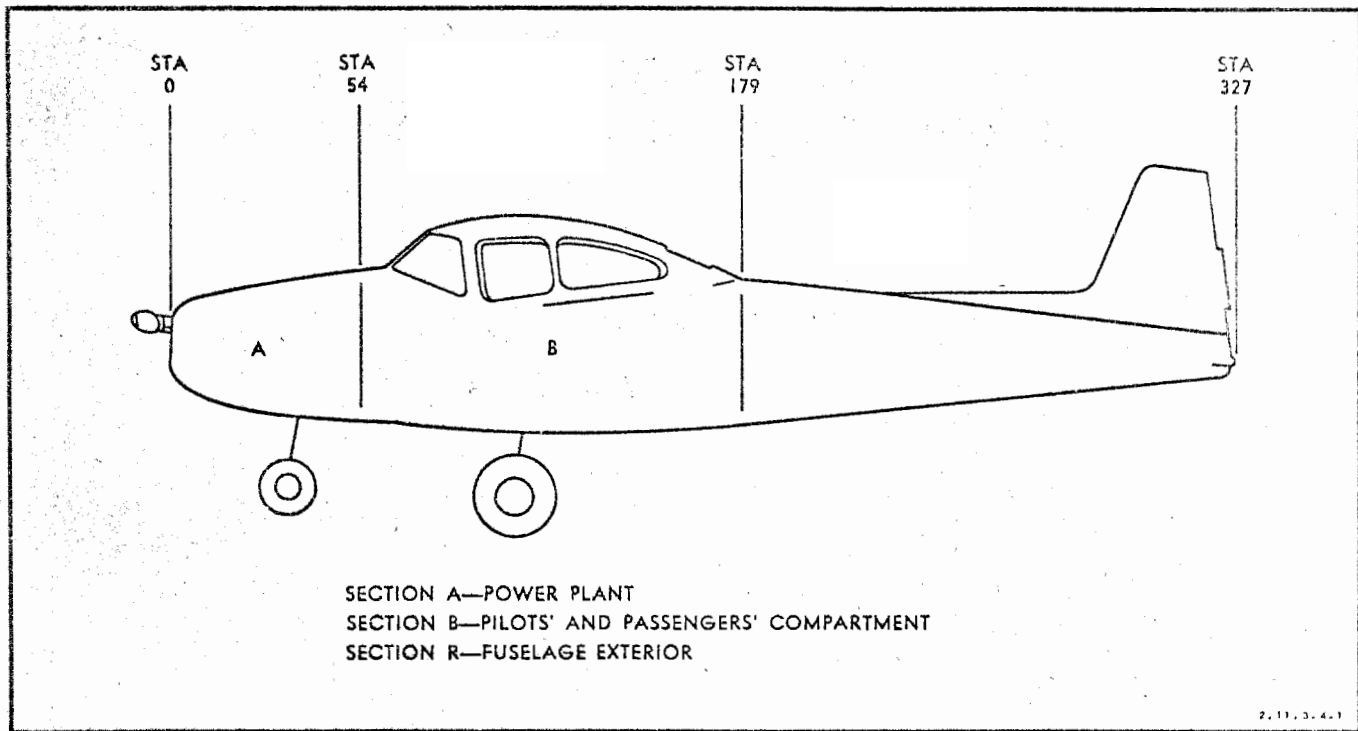
Figure 1. Sectional Breakdown Diagram
